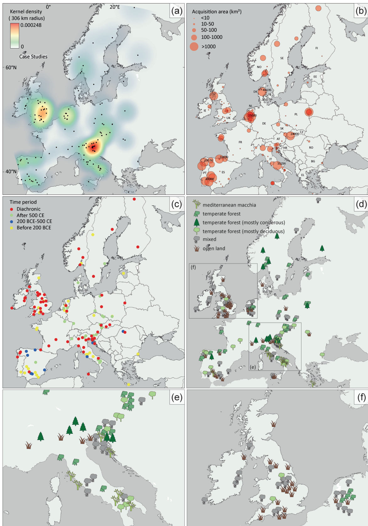
FIGURE 3 | Maps of the European case studies: (a) case studies distribution and kernel density (306 km sigma). Density is expressed in units/km²; (b) size of LiDAR acquisition areas. AT=Austria; BG=Bulgaria; DE=Germany; DK=Denmark; EE=Estonia; EL=Greece; ES=Spain; FI=Finland; FR=France; HR=Croatia; IE=Ireland; IT=Italy; NL=the Netherlands; NO=Norway; PL=Poland; PT=Portugal; RO=Romania; SE=Sweden; SI=Slovenia; SK=Slovakia; UK=United Kingdom; (c) investigated archaeological period; (d) vegetation types in the study areas with a focus on (e) Italy, Slovenia and Austria and (f) the United Kingdom, Ireland and the Netherlands.
